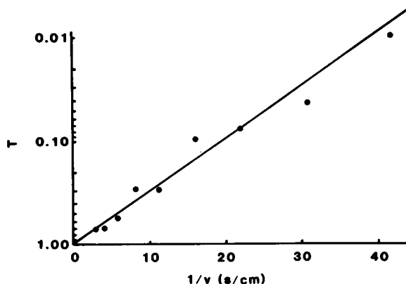
FIGURE 1 Velocity dependent magnetic capture of ferritin-conjugated 1- \mu m diam latex spheres in a 7 T (70 kG) field. The fraction of recovered particles that was passed by the HGMS filter, the transmittance T , is shown on an inverted logarithmic scale vs. the reciprocal of the buffer flow velocity, for purposes of comparison with theory (see text). The column had a cross-sectional area of 0.64 cm 2 and flow rates from 0.9–9.3 ml/min were used. The wire matrix occupied 4% of the bed volume.
