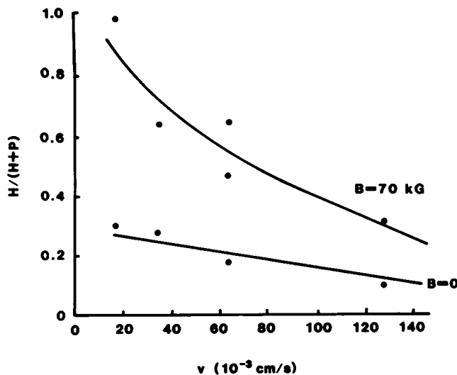
FIGURE 2 Velocity-dependent magnetic capture of immunoferritin-labeled hydrophilic beads, 5–50 \mu m diam. The column had a cross-sectional area of 0.29 cm 2 and contained 1.3 g of 25- \mu m wire that occupied 4% of the bed volume.
